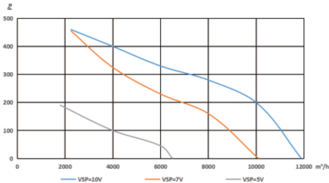
Performance Curve
